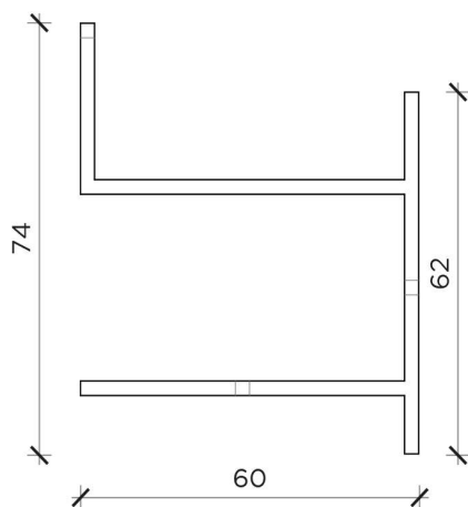
FRONTE | FRONT
