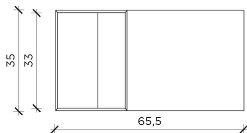
FRONTE | FRONT
