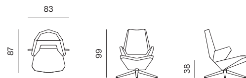
ARMCHAIR WITH WOODEN BASE dimensions 83 x 87 x 99 cm
