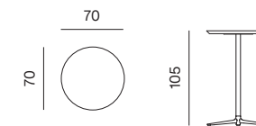
BAR TABLE dimensions \varnothing 70 / 60 \times 60 / 70 \times 70 / \times 105 cm
