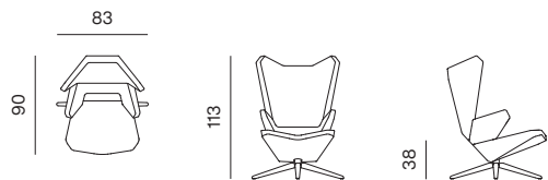
LOUNGE CHAIR dimensions 83 x 90 x 113 cm
